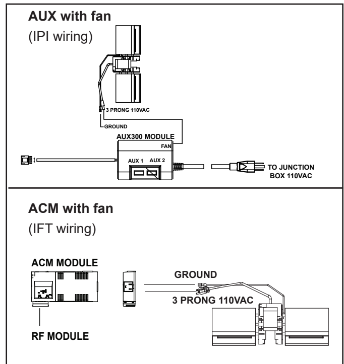
Figure 5 AUX/ACM Wiring
